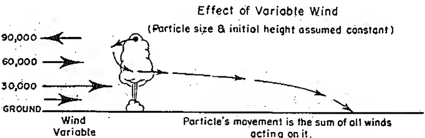
Figure 3. Factors affecting distribution of radioactive particles.
